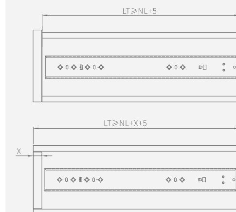
Slide Mounting Chart(mm)
