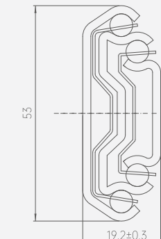
Cross Section of Slide
