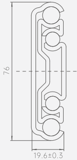
Cross Section of Slide
